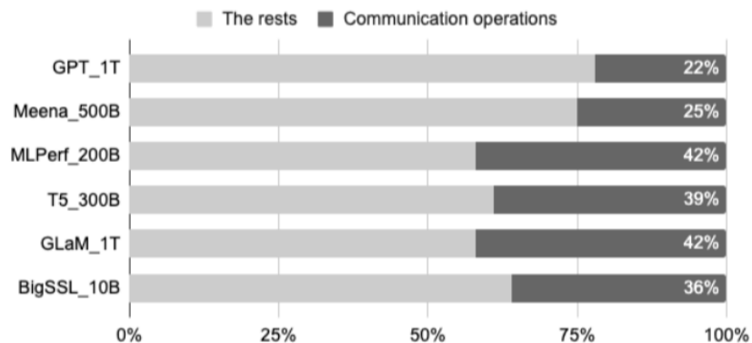
Figure 1: Training step time breakdown of large models. The models run on 128 - 2048 TPU chips depending on the model size. Details on the large models can be found in Section 6.
