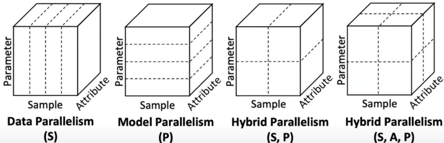
Example parallelization strategies for convolution
